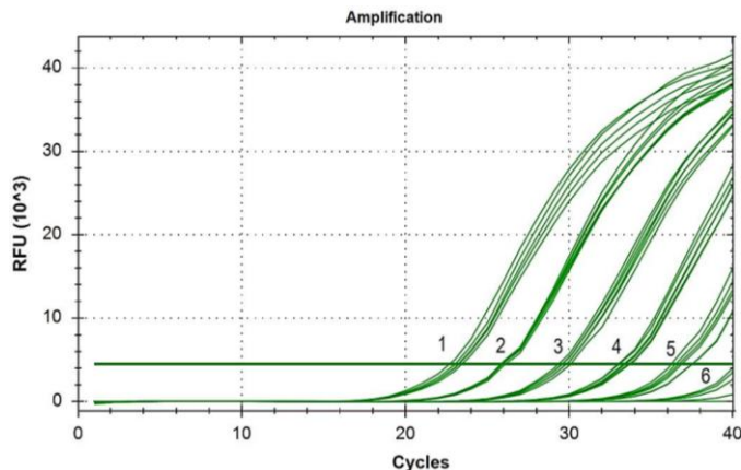
Figure 12. Detection limit of qPCR. Signals 1-6, the results of qPCR for 10 ng, 1 ng, 0.1 ng, 0.01 ng, 1 pg and 0.1 pg DNA per reaction, respectively.
